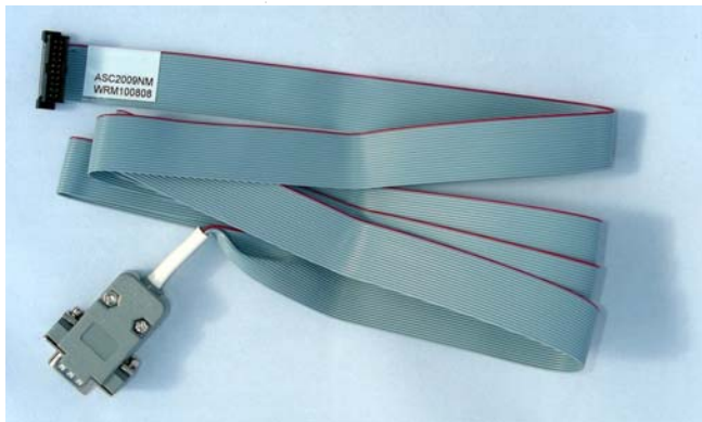
ASC2009NM NULL MODEM Cable, Diagnostics & Programming, 20 pin board level connector to DB9 - For use between Plus radio to board level serial radio
