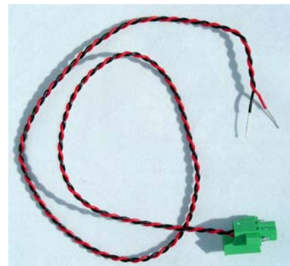
ASC2402PT Plus Power Adapter Cable Assembly, 24ga red and black, with front 2-pin connector, 24" length - For use by a Plus radio or new FGR2 enclosed radio
