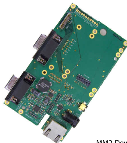
MM2-Development Board
